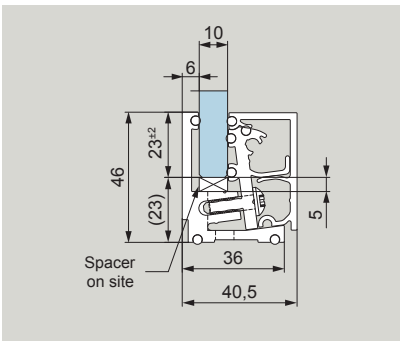
46/36 profile 46 mm visible height 10 – 13.5 mm material thickness
