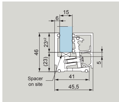
46/41 profile 46 mm visible height 14 – 18 mm material thickness
