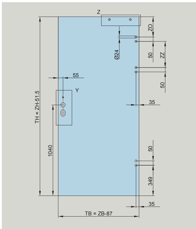
For locks and hinges up to frame height of 2201 mm to 3000 mm
