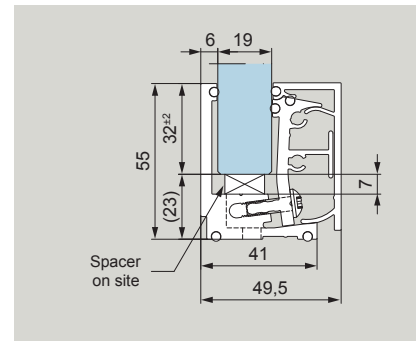
55/41 profile 55 mm visible height 16 – 19 mm material thickness
