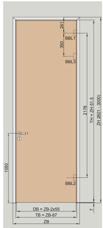
Size 3 frame height: 2601 – 3000 mm frame width: 600 – 1410
