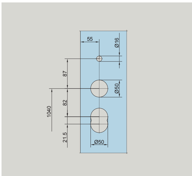
Detail Y Preparation for lock
