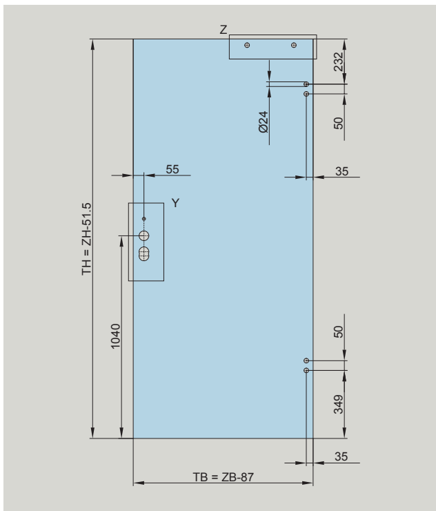
For locks and hinges up to frame height 2200 mm
