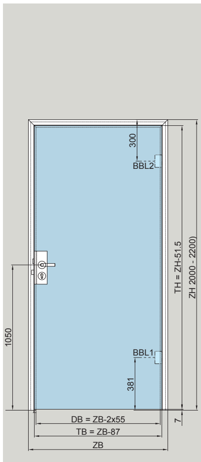
Size 1 frame height: 2000 – 2200 mm frame width: 600 – 1410
