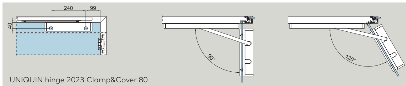
UNIQUIN hinge 2023 Standard 130
