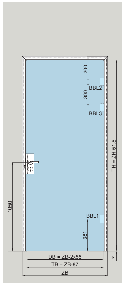
Size 2 frame height: 2201 – 2600 mm frame width: 600 – 1410
