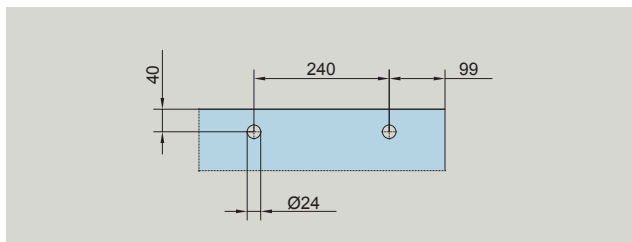
Detail Z Preparation TS 98
